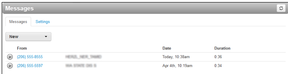
Figure 2-4. Messages Page
